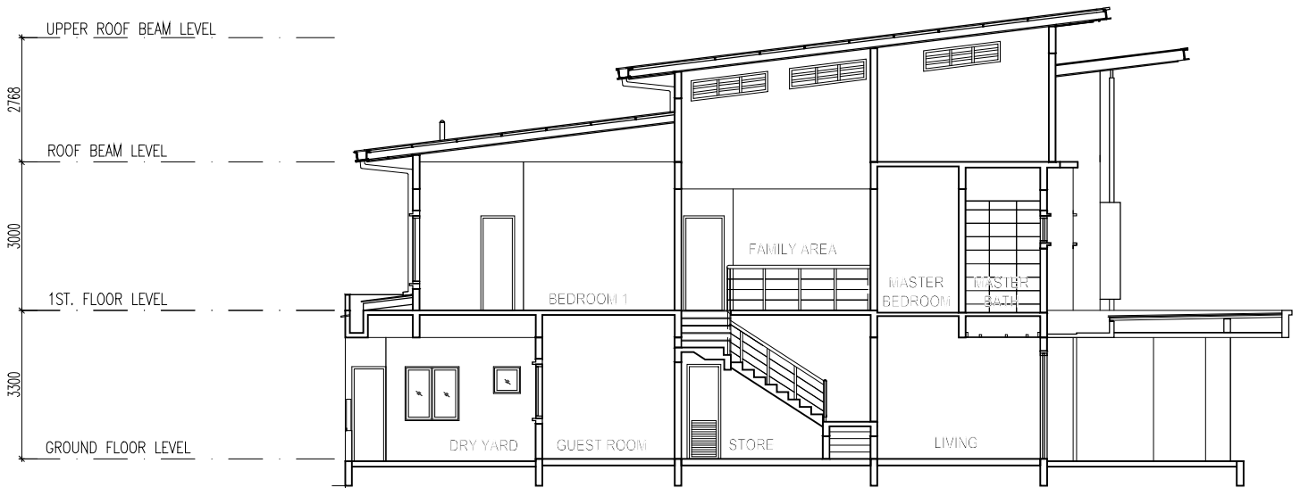
SECTION B-B
