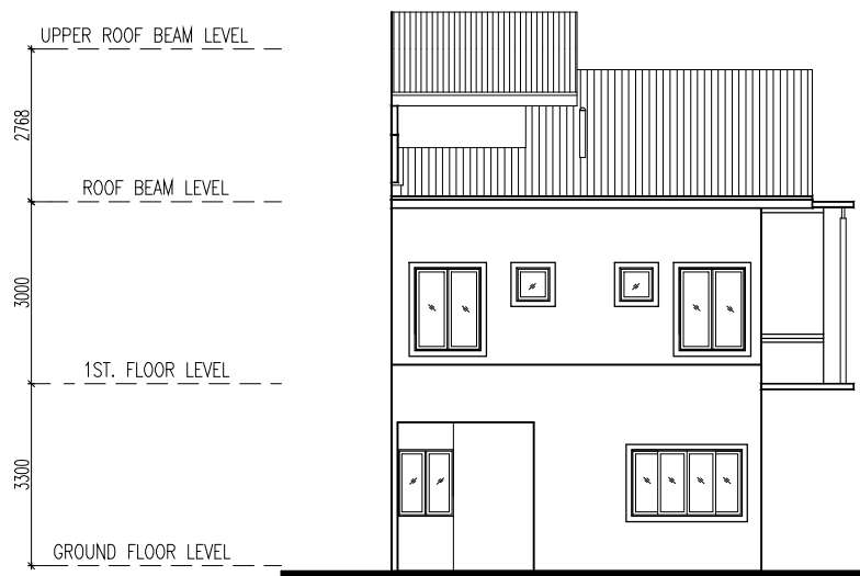
REAR ELEVATION
